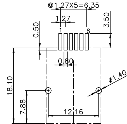
PC Board Layout Component Side Shown PC Board Thickness=1.6mm Tolerance±0.05
